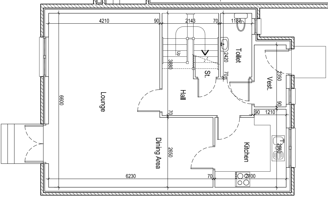
Ground Floor Plan (57.84m 2 ) Total Floor Area (117.17m 2 )
